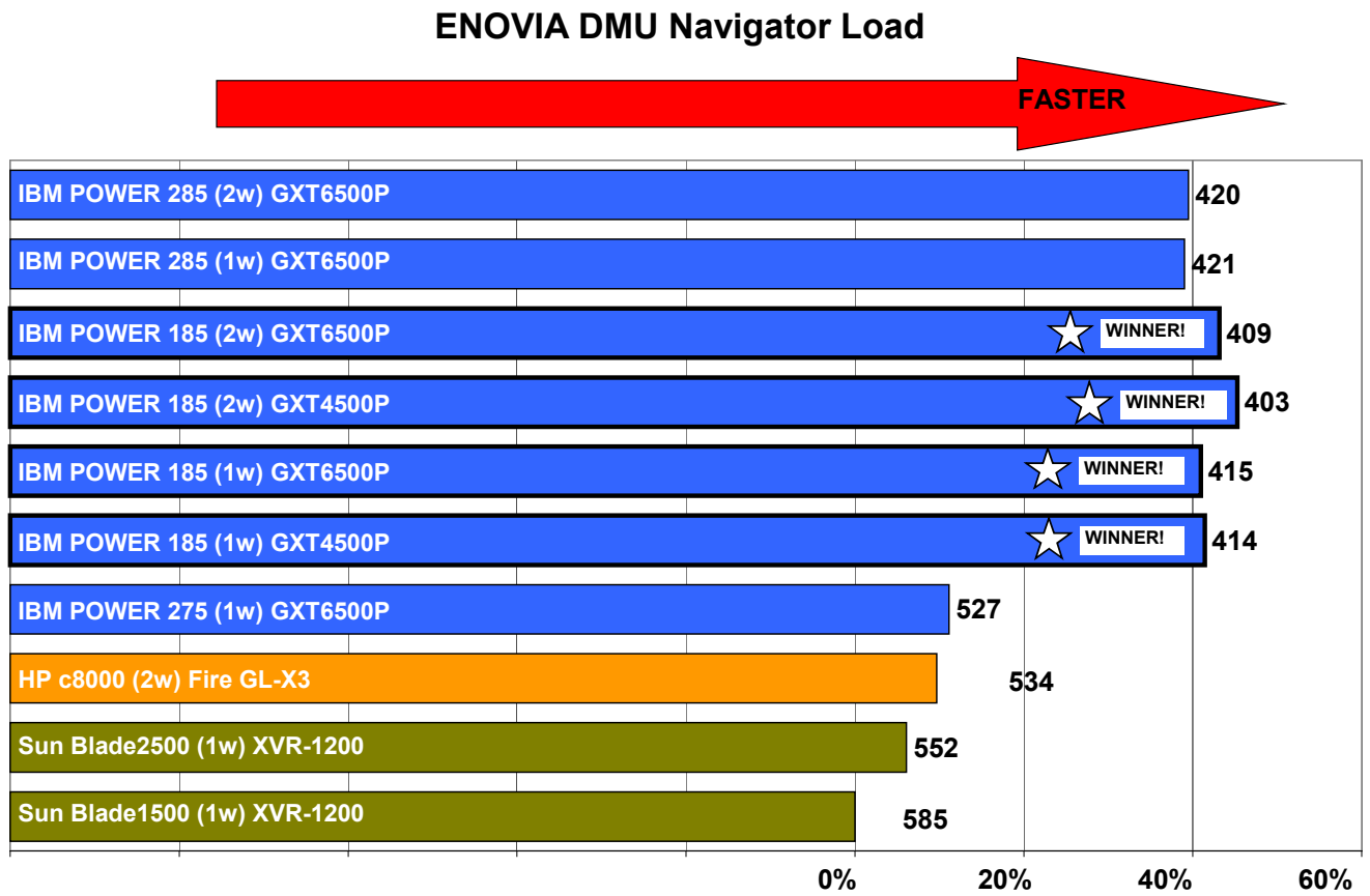
Chart 22 – ENOVIA DMU Navigator Load Throughput Relative to Slowest Machine Test time in seconds shown next to bars (smaller numbers faster) Longest bar wins! (★)
